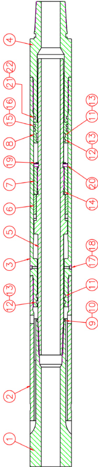
LEE OILFIELD SERVICE 3 5/8 O.D. x 1.8 I.D. TESTING JAR
