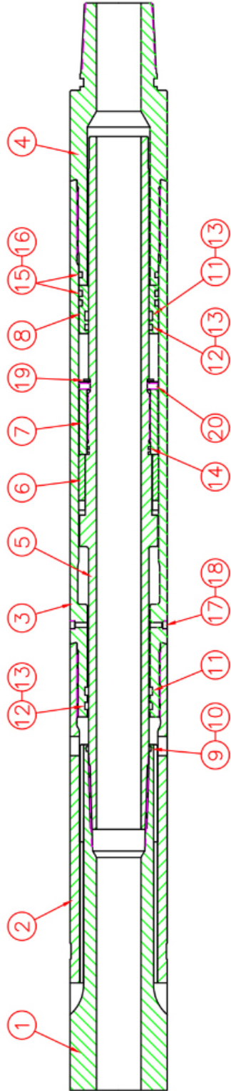
LEE OILFIELD SERVICE 5 O.D. x 2.3 I.D. TESTING JAR
