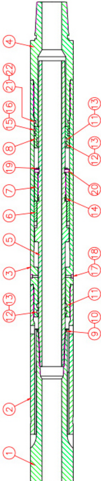
LEE OILFIELD SERVICE 3 7/8 O.D. x 1 7/8 I.D. TESTING JAR
