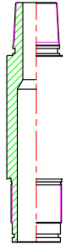
BOTTOM SUB PART #: FJ-3875BB-04
