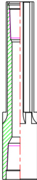
MALE SPLINE PART #: FJ-3875BB-01
